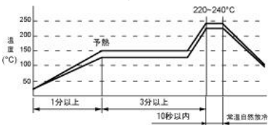
Reflow Soldering Recommended Conditions
