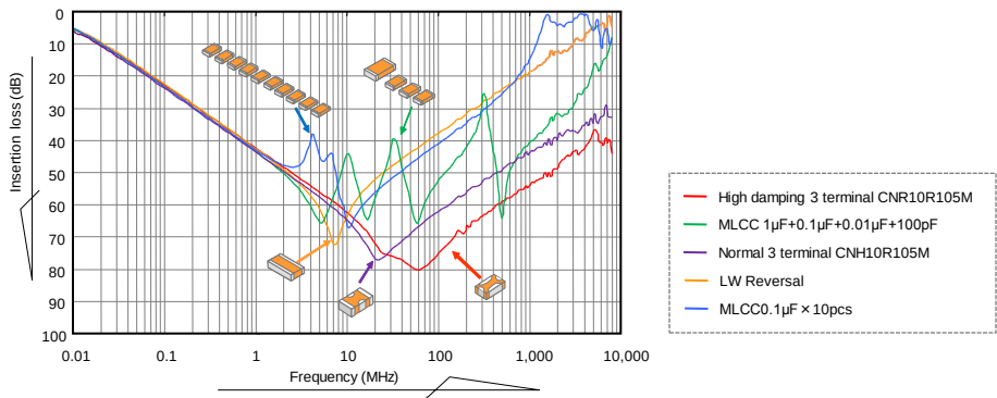
Insertion Loss Characteristics (Reference)
