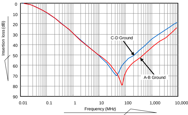
Insertion Loss Characteristics (Reference)
