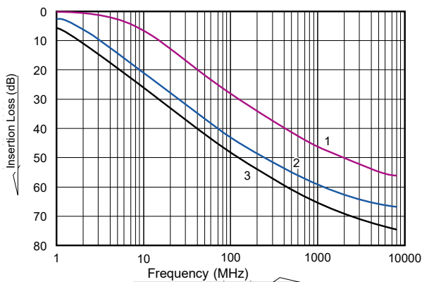
FTT30 Type Insertion Loss Data
