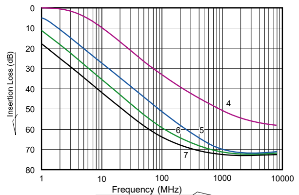
FTT40, FTT41 Type Insertion Loss Data
