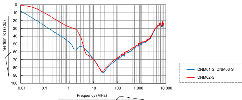
Insertion Loss (Reference)
